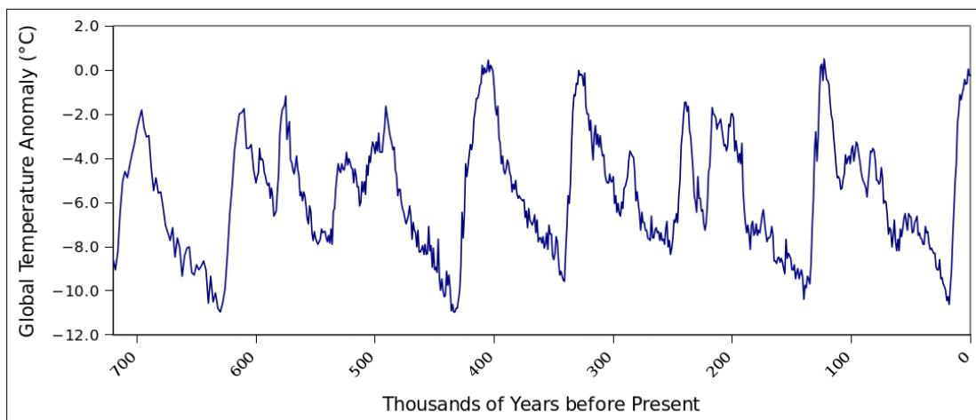
Temperature Reconstructions using deep sea sediment cores. (Raymo, 2005) From "The Inconvenient Skeptic" 2011 p42, by John Kehr http://theinconvenientskeptic.com/
