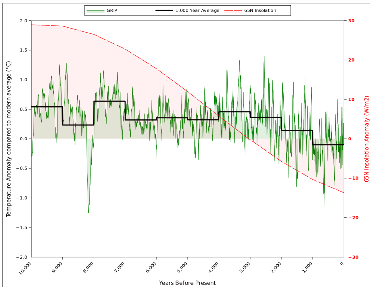
Greenland Ice Core Project –Temperature Reconstruction – “Falling for 3000 Years” From “The Inconvenient Skeptic” p 115 by John Kehr 2011, http://theinconvenientskeptic.com/
